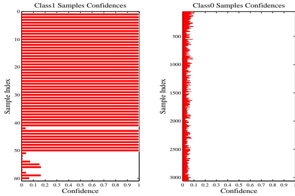
Figure 3. Confidence scores obtained by the class1 (left) and class0 (right) samples from the DLS ensemble trained with the entire artificial data set.
