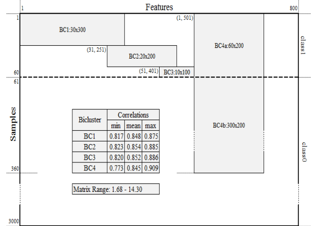
Figure 2. Characteristics of the artificial database used for testing. There are 4 biclusters embedded in the matrix, but only biclusters 1, 2 and 3 are discriminative, because, contrarily to bicluster 4, they are embedded only within class1 samples.
