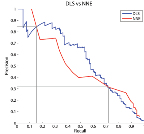
Figure 5. Comparison of the results obtained by DLS and NNE.
