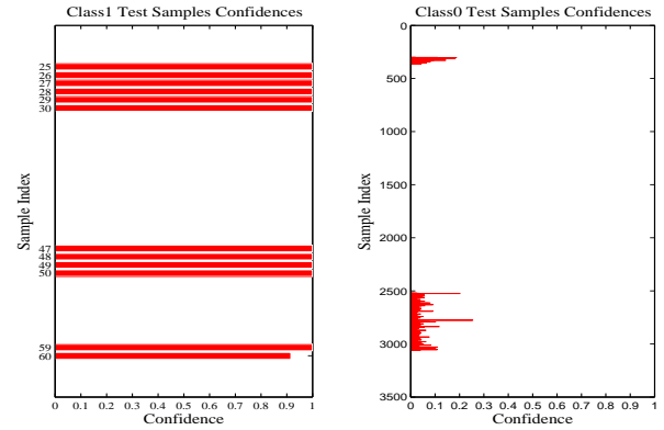
Figure 4. Confidence scores obtained by the class1 (left) and class0 (right) held-out test samples from the DLS ensemble trained with the remaining 80% of the artificial data set.
